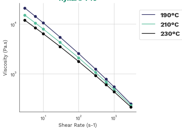
Viscosity-shear rate Kynar® 740
